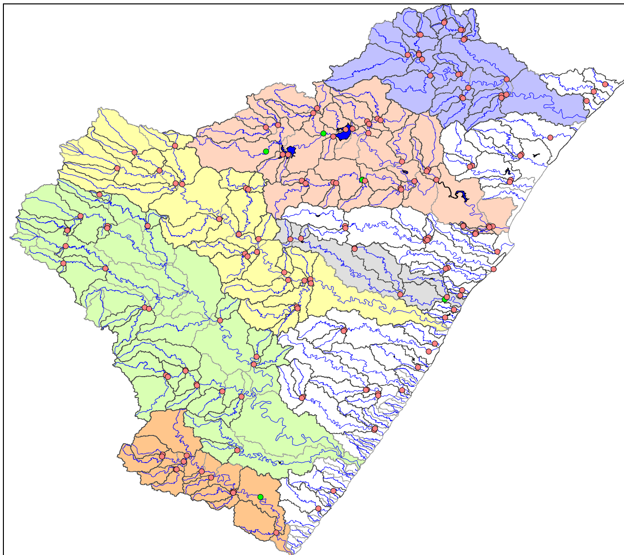
Figure 3.1 The Mvoti to Umzimkulu Classification Project visual setup in SPATSIM
